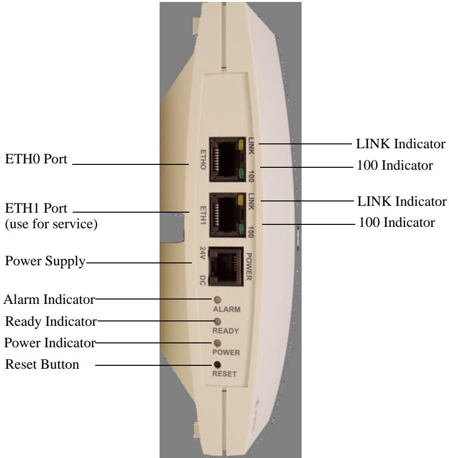
Figure 11 KIRK Wireless Server 600v3 - Faceplate
